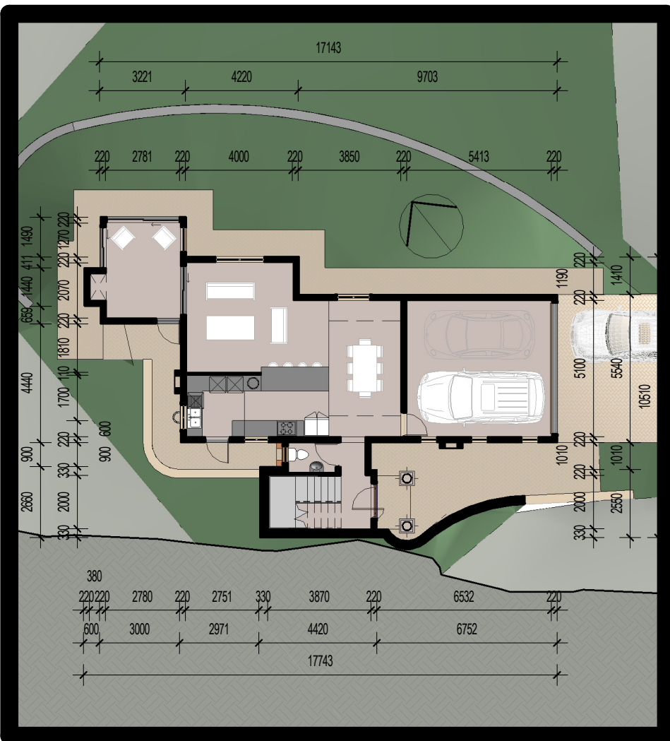
1 05 - Ground Floor 1 : 200
