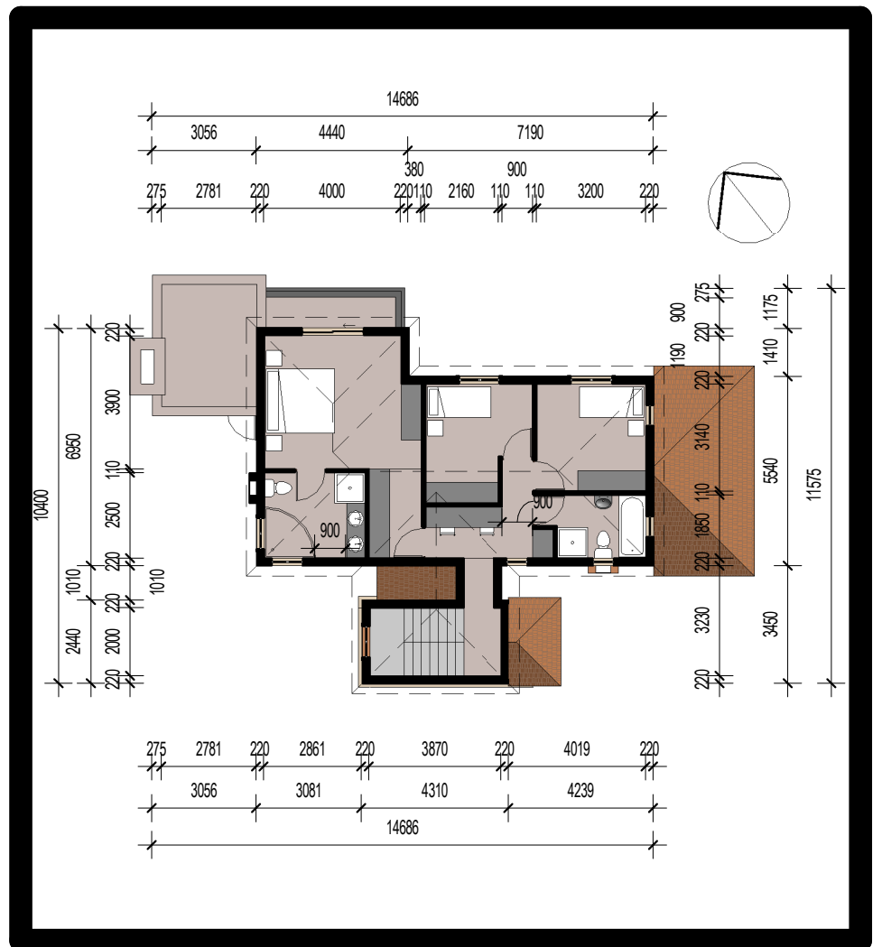
2 10 - First Floor 1 : 200
