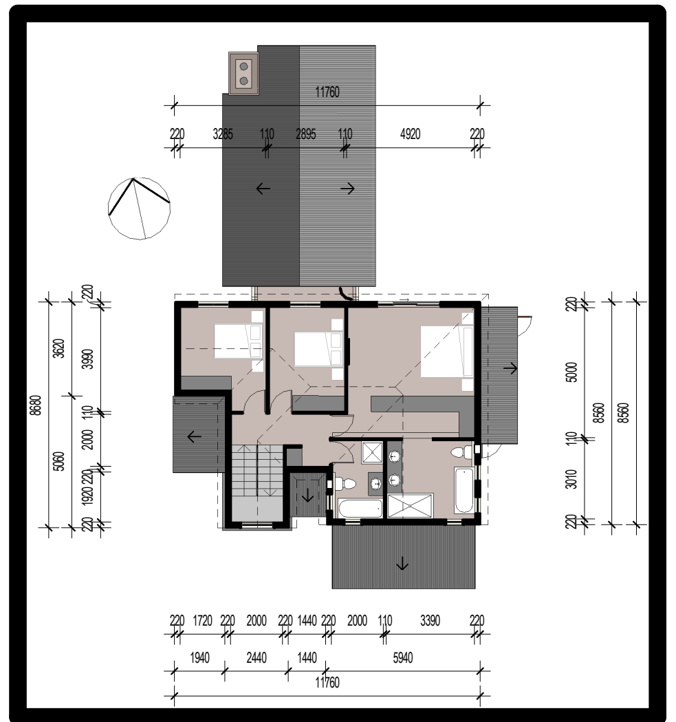
10 - First Floor
