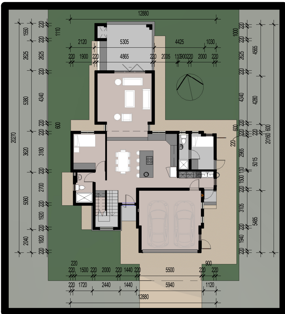
05 - Ground Floor
